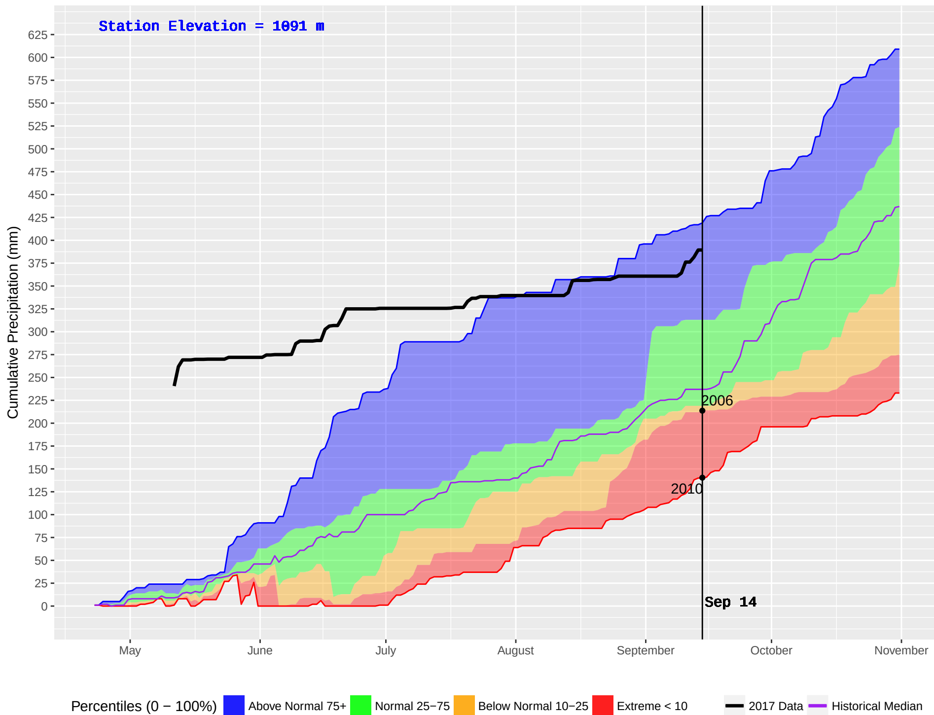
BIG MOUTH 2 (868) : Historical (2004–2016) and Current (2017) Noon Cumulative Precipitation
