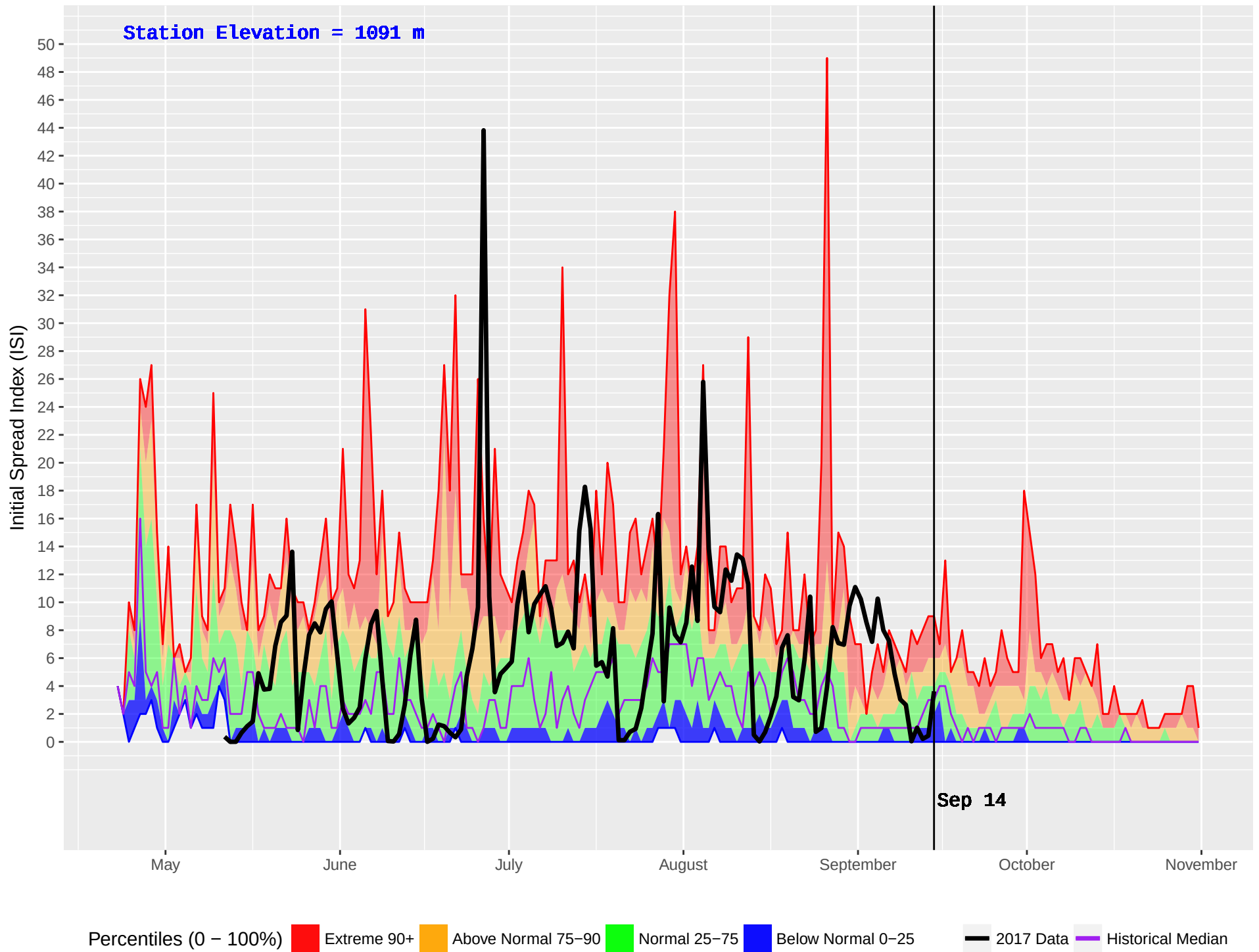
BIG MOUTH 2 (868) : Historical (2004–2016) and Current (2017) Noon Initial Spread Index (ISI)
