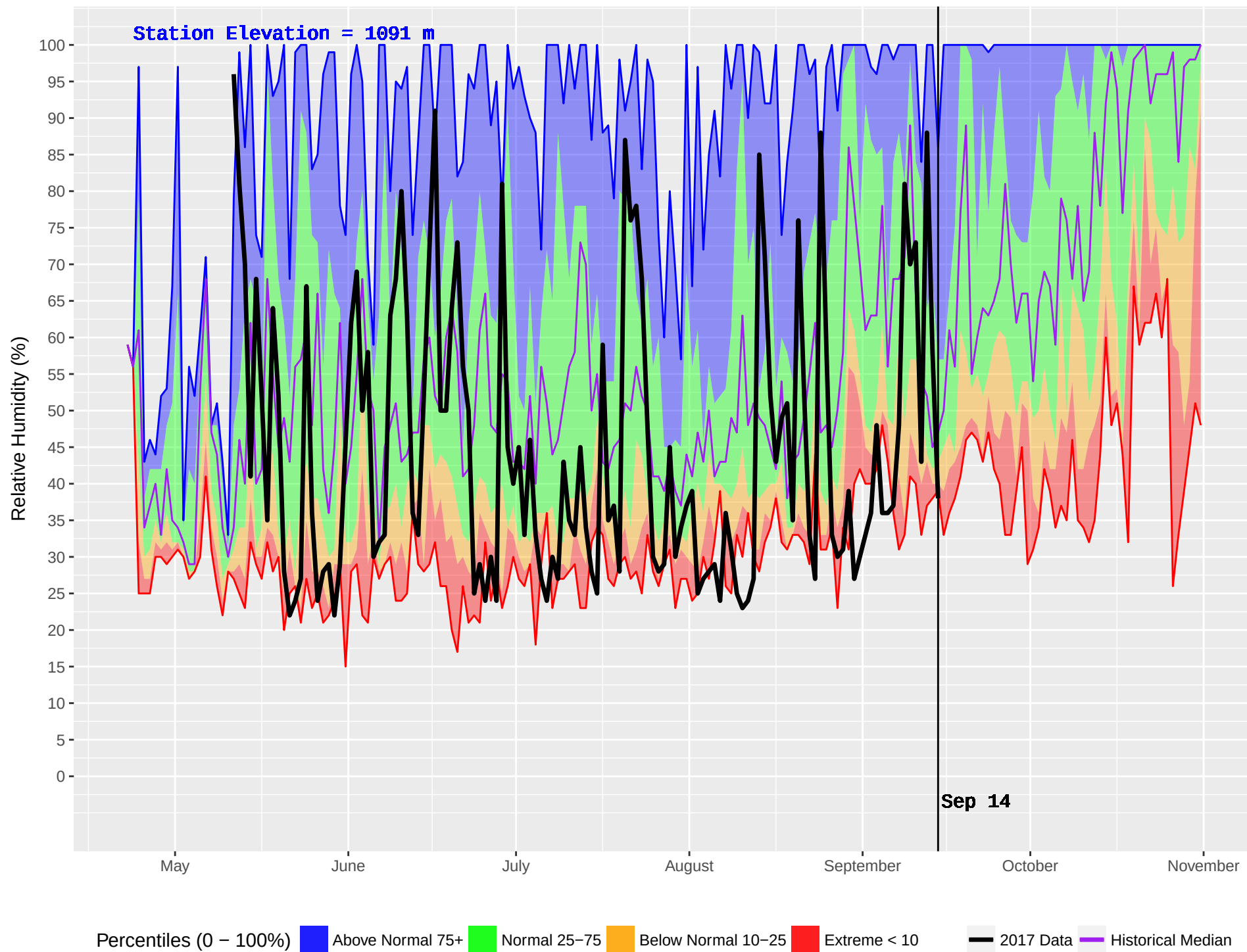
BIG MOUTH 2 (868) : Historical (2004–2016) and Current (2017) Noon Relative Humidity
